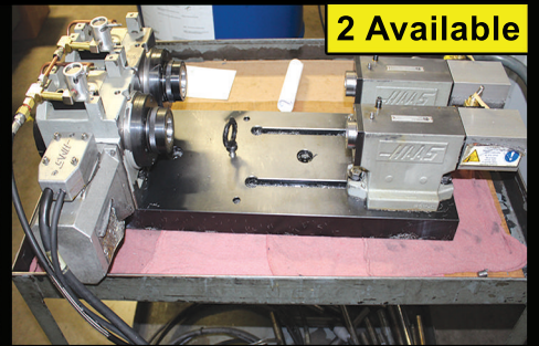
HAAS HA2TS & (2) TAILSTOCKS
